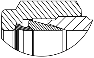
Note A - Detail View
